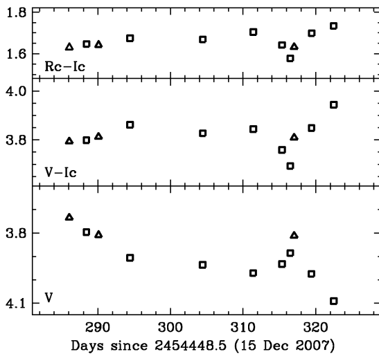
Fig. 4. A portion of the light curve shown in Figure 2 that includes the brightening at the day \sim 315 .
